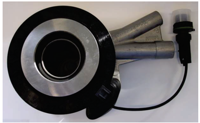
Fig. 4: 3182 600 101 with travel sensor
